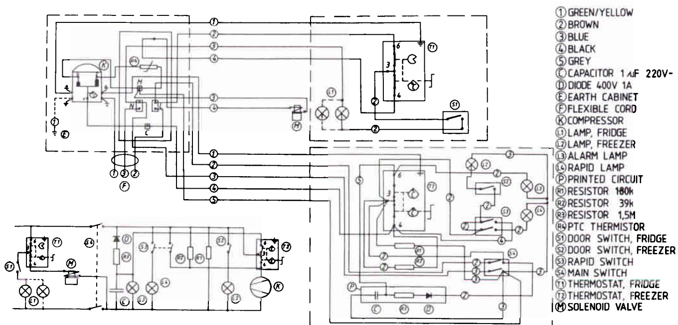
WIRING DIAGRAM 294 14 18
