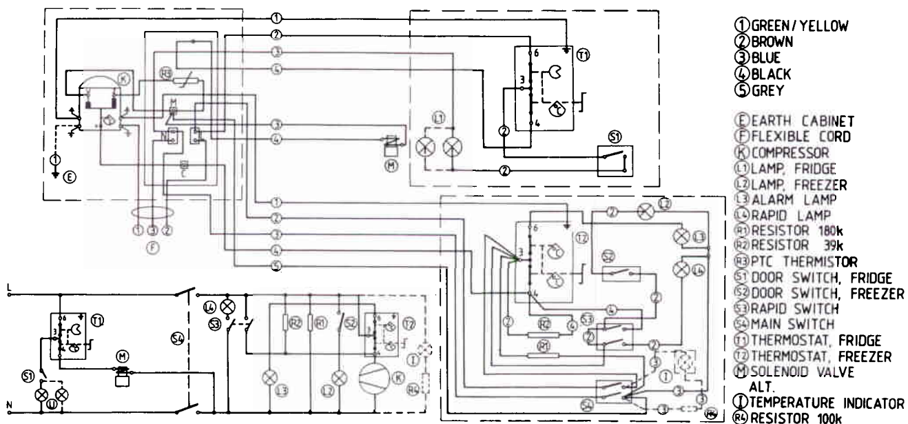
WIRING DIAGRAM 294 06 99
